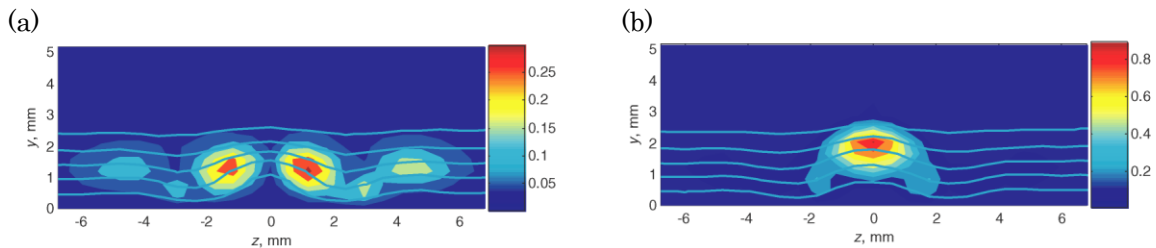
Fig. 2. Disturbances near the roughness element, at x - x_0 = 30 mm for (a) sinusoidal and (b) varicose types of instability. Filled contours show r.m.s. amplitude of the secondary high-frequency disturbances ( \tilde{u} in m/s). Lines depict contours of mean velocity at levels of 15, 30 ... 75% of U_\infty .
