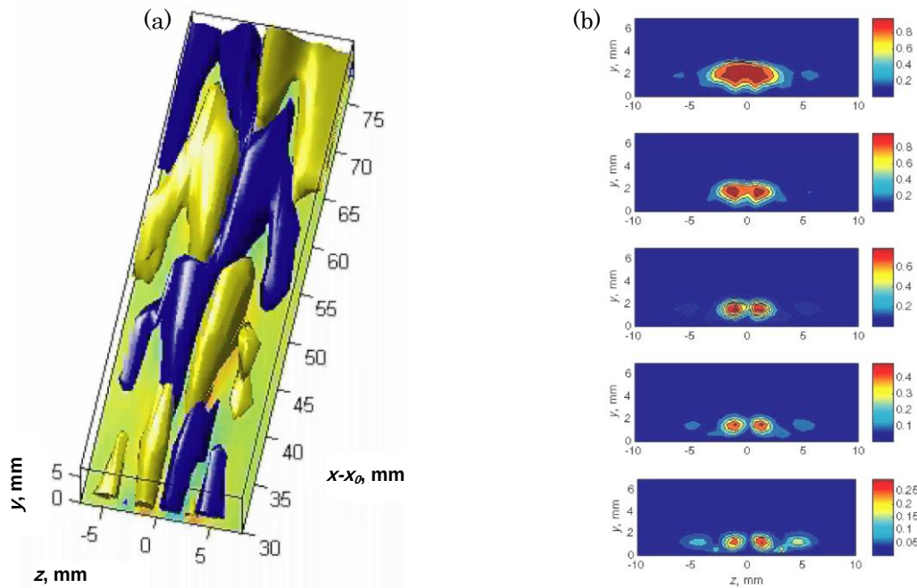
Fig. 3. Initial development of the sinusoidal instability mode. (a) isosurfaces of the instantaneous time-periodic velocity ( \tilde{u}/U_\infty = 0.75\% , yellow; \tilde{u}/U_\infty = -0.75\% , blue); (b) contours of r.m.s. velocity amplitude at streamwise stations 30, 42, 54, 66 and 78 mm, increasing from bottom to top.
