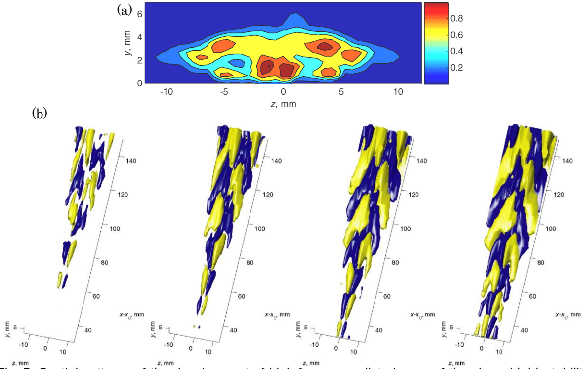
Fig. 5. Spatial patterns of the development of high-frequency disturbance of the sinusoidal instability. (a) contours of r.m.s. velocity amplitude at x - x_0 = 114 mm; (b) isosurfaces of time-periodic velocity \tilde{u} : \pm 6.4\% , 2.6\% , 1.3\% , and 0.65\% of U_\infty , from left to right.
