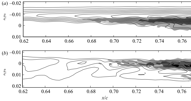
FIGURE 17. Contours of total streamwise velocity disturbance (mean and periodic part) with r.m.s. shading. Negative isolines are shown. The development of (a) 'z' and (b) 'y' modes of secondary instability is depicted.
