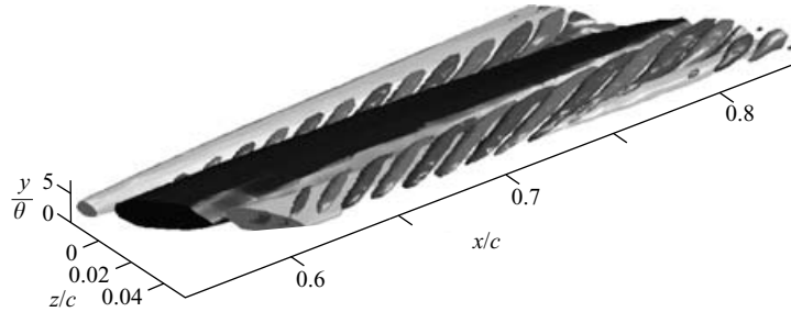
FIGURE 8. Forced periodical disturbances together with the stationary vortices of figure 4. Cases A + B are shown. Stationary disturbance isosurfaces are \pm 6\% of Q_0 , light isosurfaces of periodical disturbances: -0.5\% , dark: +0.5\% of Q_0 .
