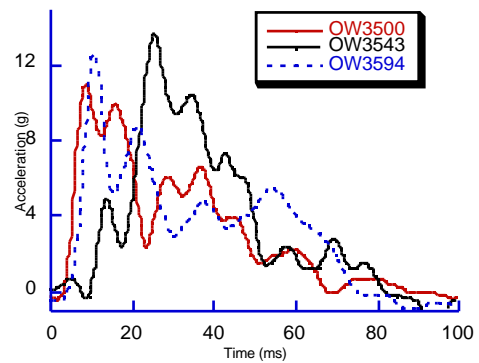
Figure A16. The acceleration pulse measured at the bottom of the B-pillar in the 100% overlap barrier test producing a delta-v between 11.0 km/h and 12.4 km/h.
