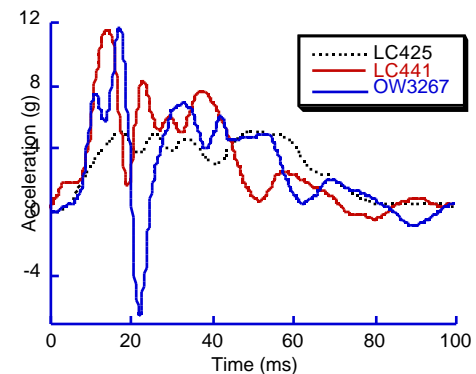
Figure A5. The acceleration pulse measured at the bottom of the B-pillar in the 40% overlap barrier test producing a delta-v between 9.4 km/h and 11.0 km/h.
