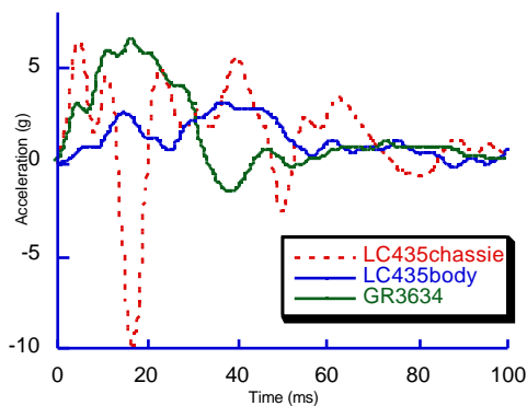
Figure A15. The acceleration pulse measured at the chassi and body in the 40% overlap barrier test
