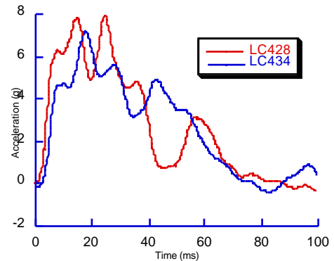
Figure A4. The acceleration pulse measured at the bottom at the B-pillar of the 40% overlap barrier test producing a delta-v of 9.3 km/h.
