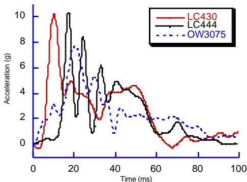
Figure A3. The acceleration pulse measured at the bottom of the B-pillar in the 40% overlap barrier test producing a delta-v between 7.9 km/h and 8.9 km/h.
