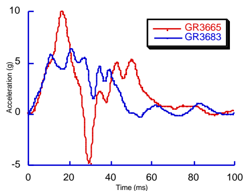
Figure A12. The acceleration pulse measured at the bottom of the B-pillar in the 40% overlap barrier test producing a delta-v of 7.8 km/h and 8.5 km/h.
