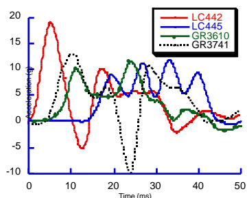
Figure 5. The crash pulses cars built with good low speed crash performances at 40% overlap at impact velocity of 15 km/h.
