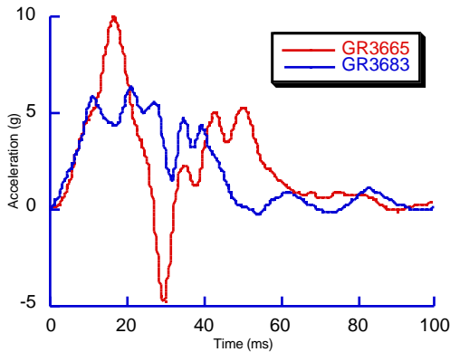
Figure A14. The acceleration pulse measured at the bottom of the B-pillar in the 40% overlap barrier test producing a delta-v of 9.4 km/h and 10.6 km/h.
