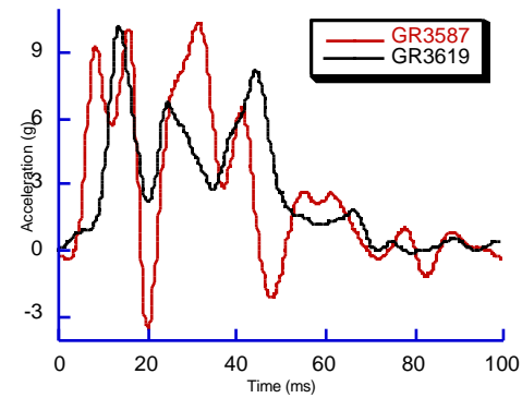
Figure A11. The acceleration pulse measured at the bottom of the B-pillar in the 40% overlap barrier test producing a delta-v of 9.0 km/h and 9.1 km/h.
