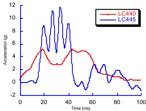
Figure A1. The acceleration pulse measured at the bottom of the B-pillar in the 40% overlap barrier test producing a delta-v of 8.9 km/h and 9.1 km/h.
