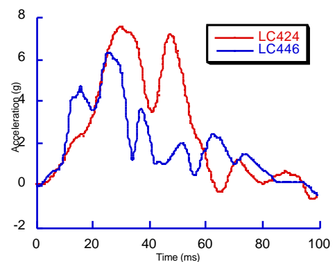
Figure A6. The acceleration pulse measured at the bottom of the B-pillar in the 40% overlap barrier test producing a delta-v of 8.2 km/h and 9.0 km/h.
