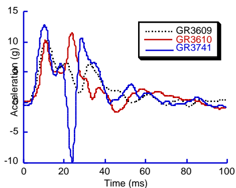
Figure A9. The acceleration pulse measured at the bottom of the B-pillar in the 40% overlap barrier test producing a delta-v between 7.2 km/h and 8.0 km/h.
