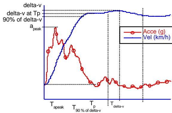
Figure 1. A Schematic drawing showing how a_{peak} , \Delta v , 90% of \Delta v , the time for these events and the duration of the acceleration pulse were identified from the graphs.
