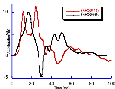
Figure 6. The crash pulses from two different cars built on the same platform at 40% overlap at impact velocity of 15 km/h.
