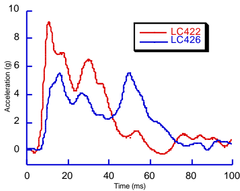
Figure A8. The acceleration pulse measured at the bottom of the B-pillar in the 40% overlap barrier test producing a delta-v of 8.0 km/h and 8.3 km/h.
