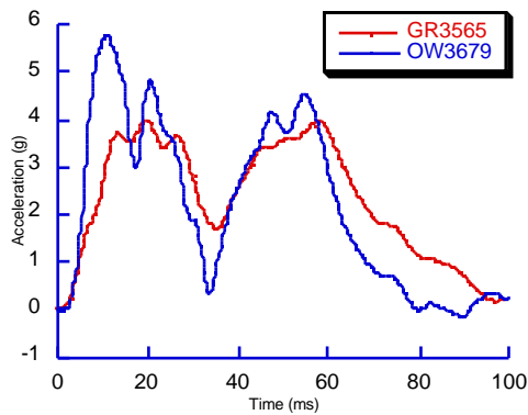
Figure A13. The acceleration pulse measured at the bottom of the B-pillar in the 40% overlap barrier test producing a delta-v of 8.0 km/h and 8.2 km/h
