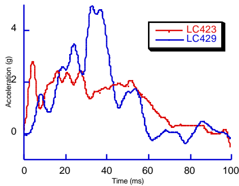
Figure A7. The acceleration pulse measured at the bottom of the B-pillar in the 40% overlap barrier test producing a delta-v of 4.3 km/h and 4.5 km/h.
