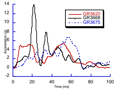
Figure A10. The acceleration pulse measured at the bottom of the B-pillar in the 40% overlap barrier test producing a delta-v between 6.9 km/h and 8.3 km/h.
