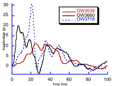
Figure A17. The acceleration pulse measured at the bottom of the B-pillar in the 100% overlap barrier test producing a delta-v between 14.0 km/h and 18.8 km/h.
