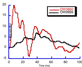
Figure 2. The crash pulses from two cars of the same make, the OW9999 built in 1983 and the OW3660 built in 1998, in a test at 100% overlap with a delta-v of 10.6 km/h and 18.6 km/h.
