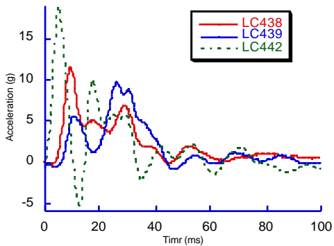
Figure A2. The acceleration pulse measured at the bottom of the B- pillar in the 40% overlap barrier test producing a delta-v between 6.6 km/h and 7.4 km/h.
